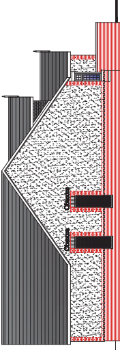
SIDE ELEVATION
